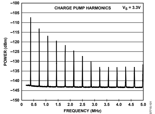
Figure 29. Output Spectrum vs. Frequency
