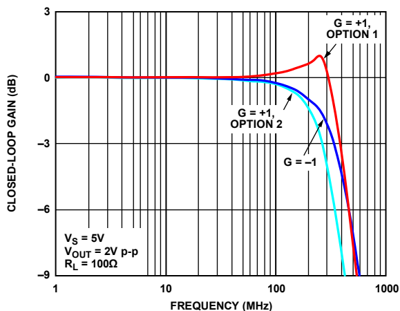
Figure 35. Large Signal, G = +1 and G = -1
